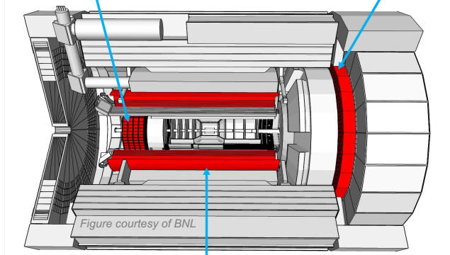
Barrel Imaging Calorimeter
